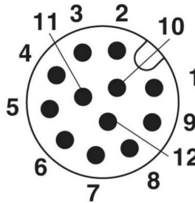
Tool Side: Pin assignment M12, 12-pos., A-coded male connector
